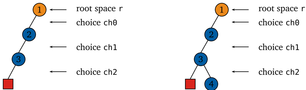
Figure 42.3: Example situations during recomputation
